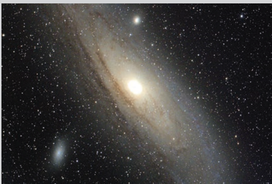
Andromeda Galaxy, M31
