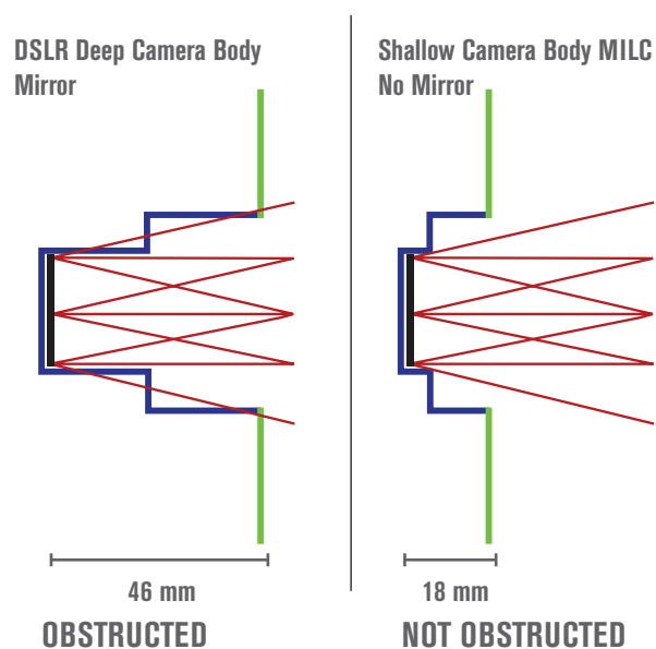
Fig. 19: The DSLR, with its deeply recessed sensor and obstructing mirror box, will block some of the RASA's light from reaching the edges of a full-frame sensor. The MILC does not have this problem.
